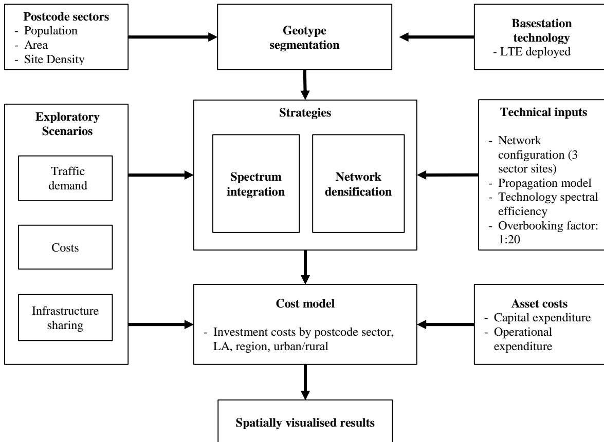
Figure 2 Sequential methodology
