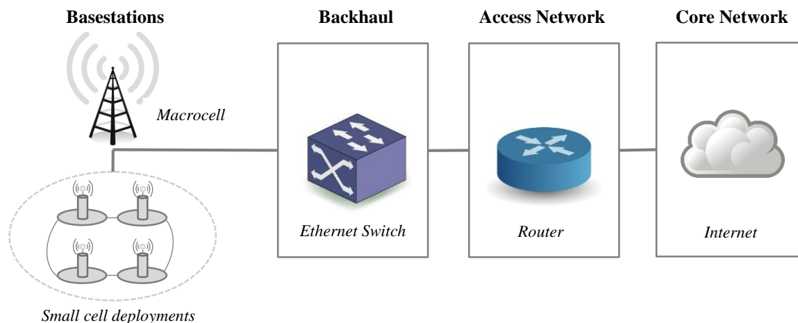
Figure 5 Network architecture
